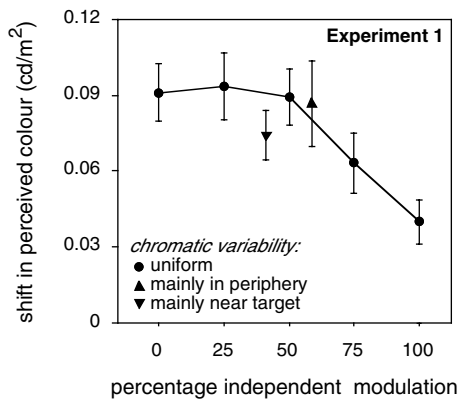
Fig. 3. Average increase in L cone stimulation from the target when settings are made with a reddish rather than a greenish background, as a function of the percentage of the modulation that was independent for the three cone types (with the 26 subjects’ inter-subject standard errors). 0% independent modulation means that only luminance is modulated. 100% independent modulation gives the maximal colour modulation. Circles: uniform distribution of modulation across the background. Triangles: gradient between 0% independent modulation for squares at the periphery and 100% independent modulation for ones near the target (triangle pointing downwards), or 0% independent modulation at the target and 100% independent modulation near the periphery (triangle pointing upwards).
