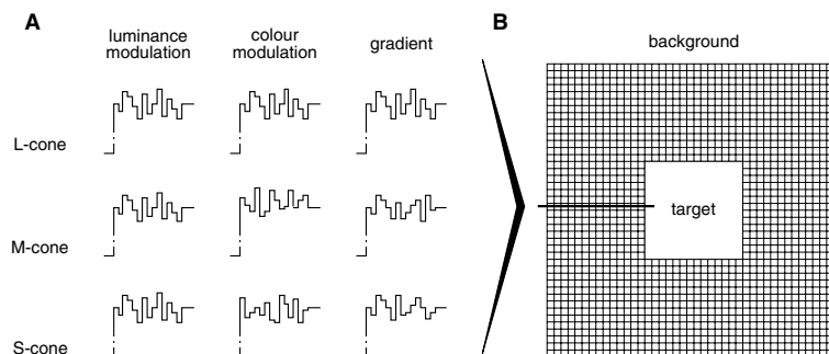
Fig. 1. Schematic representation of the stimulus configuration (B) and of the stimulation of each kind of cone by three kinds of modulation (A). Each figure in A shows the level of stimulation of one cone type as one moves along the thick line in B. The three kinds of modulation that are shown are luminance modulation (the three cones vary together), colour modulation (the three cones vary independently) and a gradient with colour modulation near the central target and luminance modulation at the periphery.
