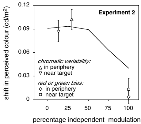
Fig. 4. Average increase in L cone stimulation from the target when settings are made with a reddish rather than a greenish background, as a function of the percentage of the modulation that was independent for the three cone types (with the 12 subjects' inter-subject standard errors). The line from Fig. 3 is also shown for comparison. Triangles: 0% independent modulation in all but the three rings of squares nearest to (triangle pointing downwards) or furthest from (triangle pointing upwards) the target, which have 100% independent modulation. Square and diamond: 100% independent modulation throughout, but only the inner (square) or outer (diamond) three rings of squares are reddish or greenish (the average chromaticity of the rest is grey).
