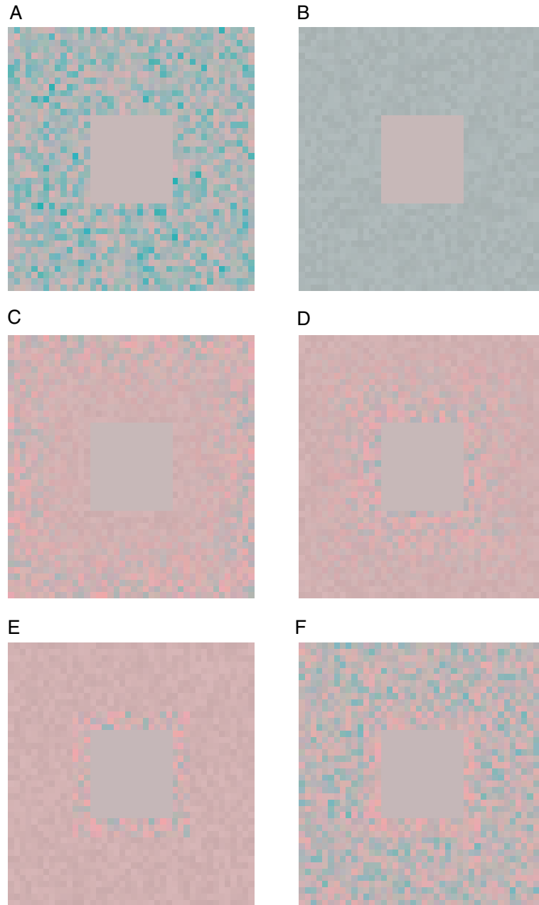
Fig. 2. Reproductions of some of the stimuli that we used. (A) Green bias; 100% independent modulation; Experiment 1. (B) Green bias; 0% independent modulation; Experiment 1. (C) Red bias; gradient with 0% independent modulation near the target and 100% independent modulation at the periphery; Experiment 1. (D) Red bias; gradient with 100% independent modulation near the target and 0% independent modulation at the periphery; Experiment 1. (E) Red bias; three rings with 100% independent modulation near the target; rest 0% independent modulation; Experiment 2. (F) Three rings with red bias near the target; 100% independent modulation; Experiment 2. (The targets for these reproductions were all set to the reference grey.)
