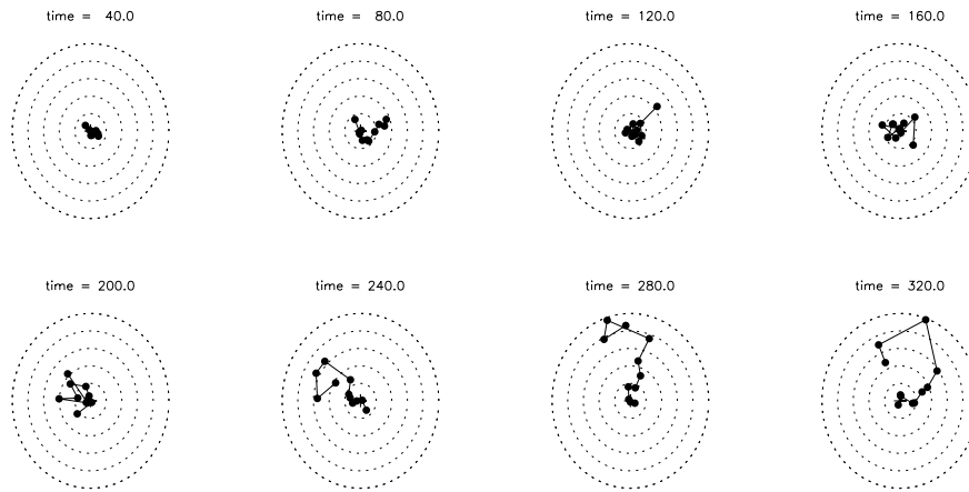
Figure 7. tip-LON diagrams at different time-steps for the simulation that has the same parameters as that in Fig. 6 except that the satellite is orbiting in the opposite sense (simulation no 7). We have binned the disc every 0.5 scalelengths in radius. There is a dotted circle every degree.
