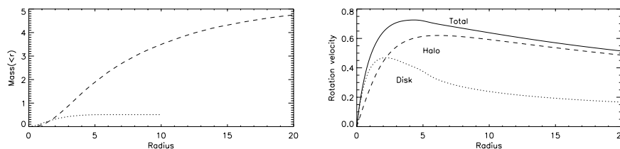
Figure 1. Mass profile and rotation curve: disc (dotted), halo (dashed) and total (solid). Simulation units are described in Section 2.2.
