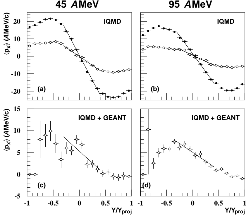
Figure 5: Average in-plane transverse momentum as a function of the rapidity normalised to the projectile rapidity. The figures on the left are for 45 AMeV data, on the right for 95 AMeV. All data is mid-central. Figures (a) and (b) are the results for IQMD events with the projection on the real reaction plane (filled circles) and on the reconstructed reaction plane with the ACM (open circles). The figures (c) and (d) show the results after the IQMD events are processed by the detector simulation, with the reconstructed reaction plane. The lines are fits of a straight line and are used to calculate the flow (see text).
