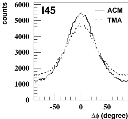
Figure 3: On the left: the distributions for the difference in azimuthal angle between the reconstructed reaction plane and the real reaction plane using the transverse-momentum analysis and the azimuthal-correlation method at 45 AMeV for IQMD data. On the right: RMS of the distributions of the difference between the reconstructed event-plane and the real event plane for the four described methods, the sphericity flow-tensor method with the mass (STM) and with 1 (ST1) in the weight factor, the transverse-momentum analysis (TMA) and the azimuthal-correlation method (ACM). The last row indicates the error in the values of that column. The methods were tested at 45 and 95 AMeV before and after the detector simulation, denoted respectively with I and G. All results are for mid-central events.
