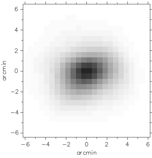
NGC5236
