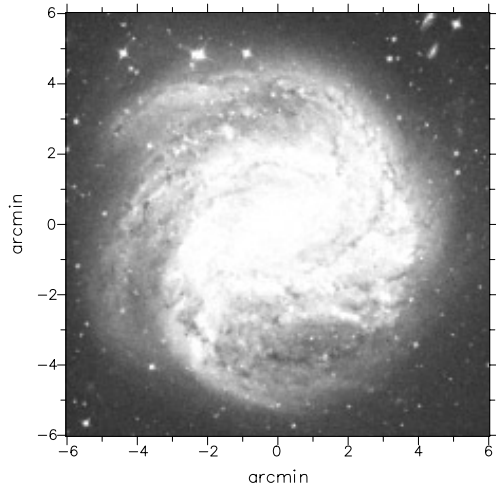
NGC5236
