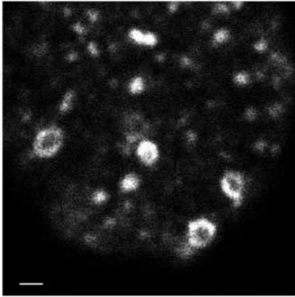
Fig. 6. Mrp2 is present in large vacuoles in nocodazole-treated cells. Hepatocyte couplets were cultured for 3 hours in the presence of 20 \mu\text{M} nocodazole. Cells were fixed and stained for mrp2. A high magnification image of the top section, taken just beneath the plasma membrane, of one half of a couplet is shown. Mrp2 is localized to large vacuoles, some with diameters of 1 \mu\text{m} , close to the basolateral membrane. Bar, 1 \mu\text{m} .
