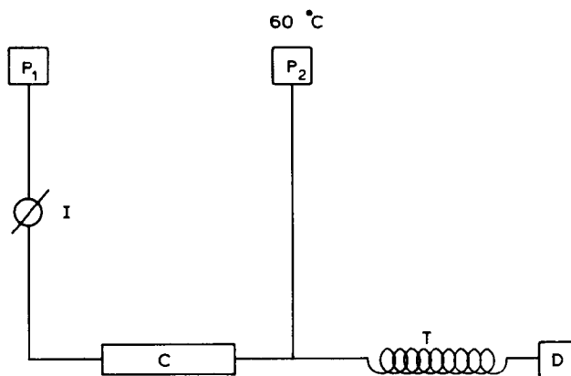
Figure 1. Schematic diagram of the chromatographic system: P 1 =pump for mobile phase; P 2 =pump for post-column reagent; I= injection valve; C= column; T=capillary tubing; D=detector.
