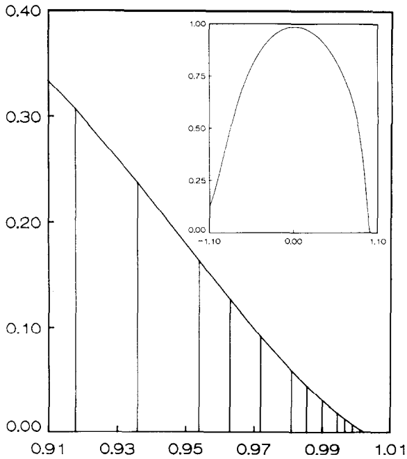
FIG. 13. The pressure p in the neighborhood of the cavitation boundary x=b . This computation is performed using a non-equidistant grid refinement. The x variable and p are scaled as in Fig. 9; M \approx 10 .
