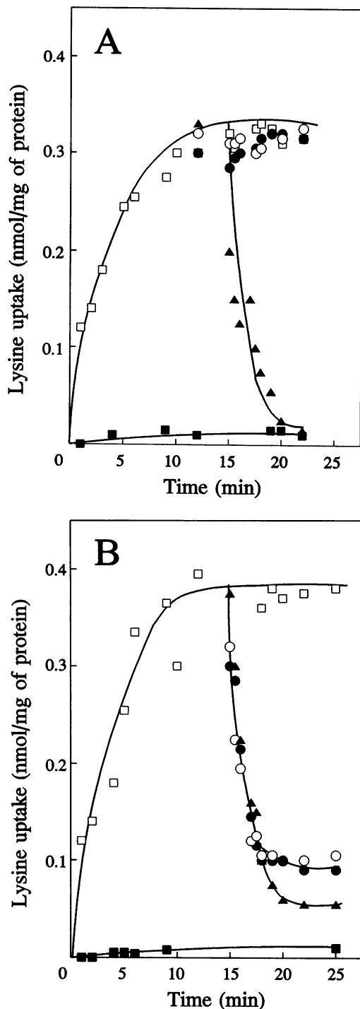
FIG. 4. Release of L-[ 14 C]lysine by the addition of a 100-fold excess of L-lysine (▲), L-arginine (●), and L-ornithine (○) by control (A) and ArcD (B) membrane vesicles. Membrane vesicles were incubated in the presence (□) and absence (■) of glucose-PQQ and allowed to accumulate L-[ 14 C]lysine for 15 min, and then the unlabeled amino acids were added. Further experimental details are given in the legend to Fig. 3.
