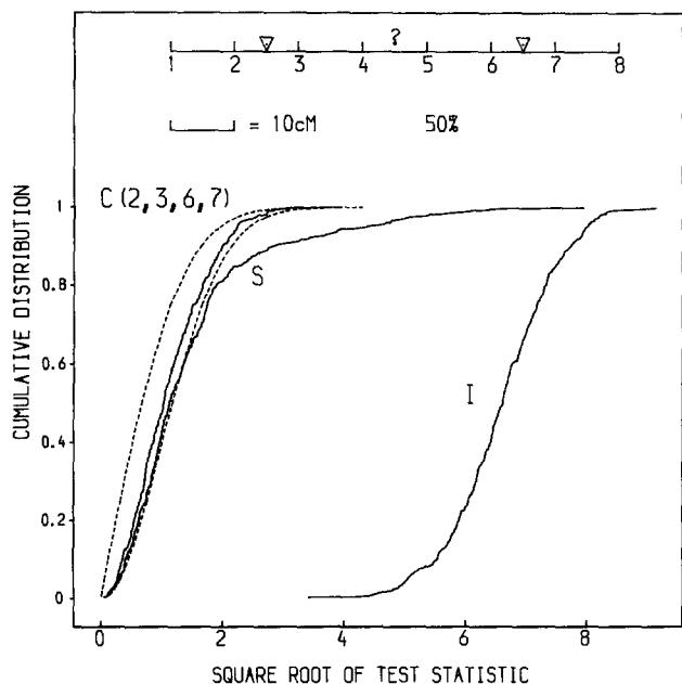
FIGURE 3.—A study of the I type error at an interval between two QTLs in coupling phase (see Figure 1 legend).
