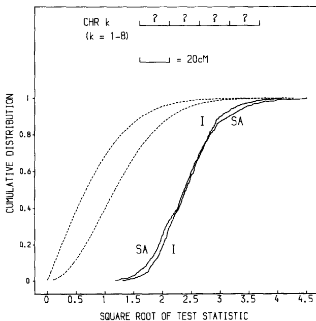
FIGURE 5.—A study of the type I error in an entire genome (see Figure 5.1 legend).
