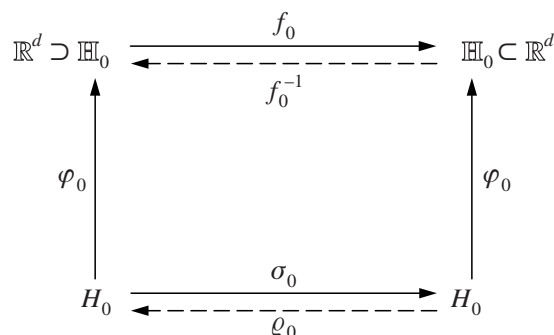
Figure 1. The abstract manifold H_0 and its embedding in \mathbb{R}^d .
