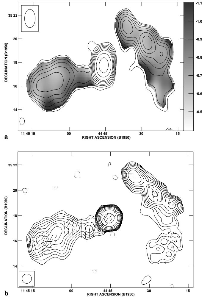
Fig. 2a and b. Radio maps of the source B1144+352 from the WENSS and the NVSS surveys. a Contour plot from the 325-MHz WENSS survey. Contour levels are at (-8, 8, 11.3, 16, 22.6, 32, 45.3, 64, 128, 256, 512) mJy beam ^{-1} . The grey scale represents the spectral index \alpha between 1400 and 325 MHz, calculated using only pixels above a 4\sigma -level in the WENSS and convolved NVSS maps. It ranges from -0.4 (white) to -1.1 (black). b Contour plot from the 1.4-GHz NVSS survey. Contours are at (-1.2, 1.2, 1.7, 2.4, 3.4, 4.8, 6.8, 9.6, 19.2, 38.4, 76.8, 307.2) mJy beam ^{-1} . Also plotted are the observed E -field polarization vectors, with a length proportional to the polarized intensity ( 1'' = 0.05 mJy beam ^{-1} ).
