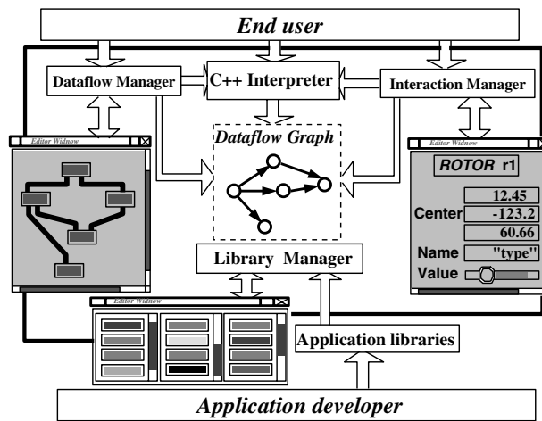
Figure 5: Architecture of the simulation and visualization system
