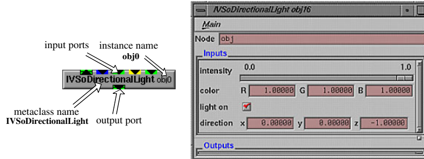
Figure 3: Left: Visual icon for a metaclass. Several graphical signs encode the ports' C++ types, by value/by reference transfer, and other attributes. Right: automatically built GUI for the metaclass
