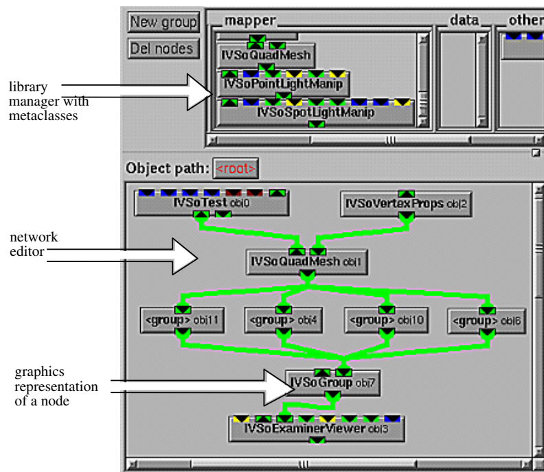
Figure 4: The network editor and the dataflow graph. Nodes are created from metaclasses shown in the library manager’s GUI.
