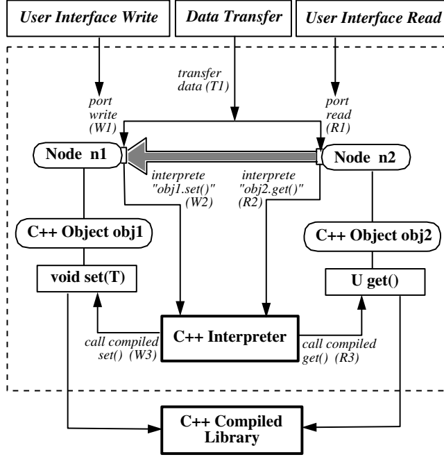
Figure 7: User interface read/write operations, data transfers between ports and the underlying C++ mechanism
