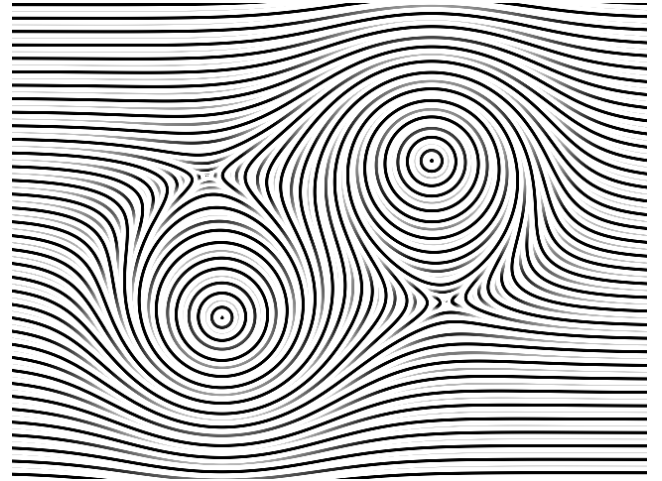
Figure 7: Dense contours
