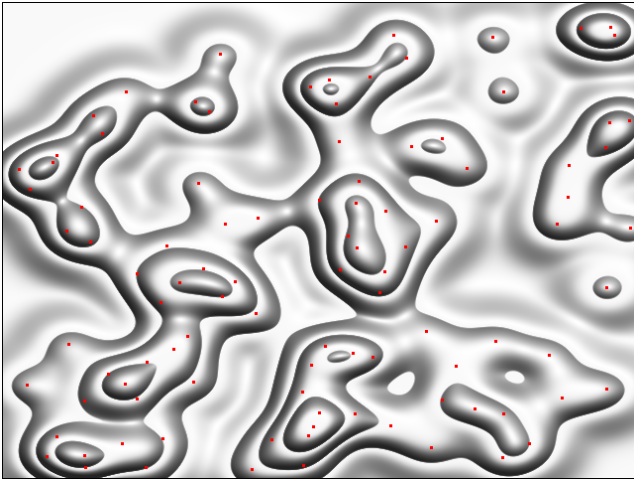
Figure 6: Nested clusters
