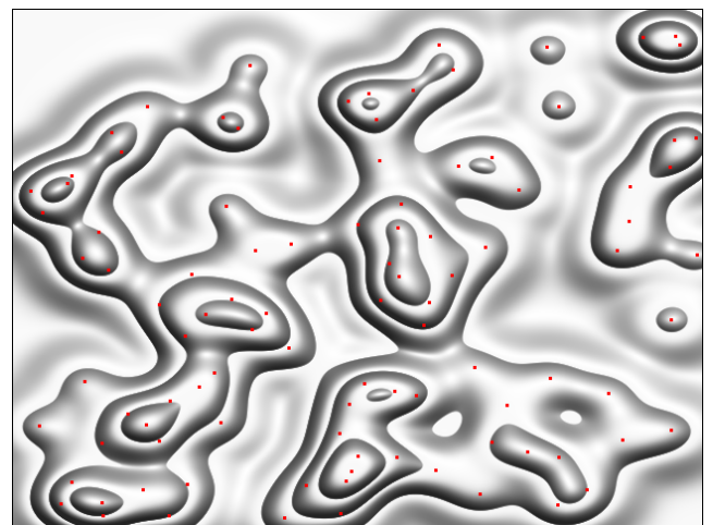
Figure 6: Nested clusters
