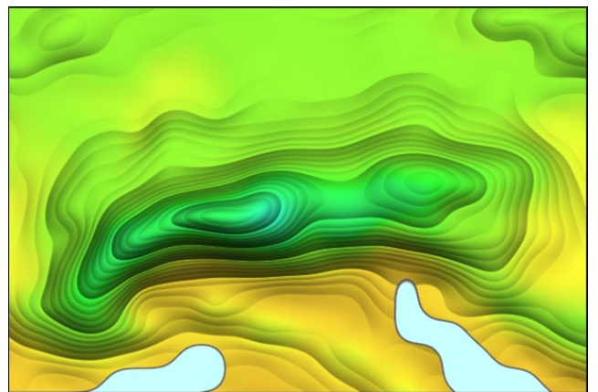
Figure 13: Average temperature (color) and precipitation (height) Alps, July
