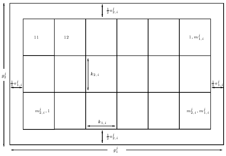
Figure 2.1: Relation between a large sheet and rotary cut formats
