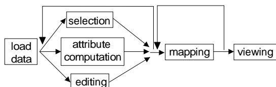
Figure 1: Operation pipeline
