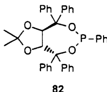
Scheme 7.22. Enantioselective conjugate addition to nitroalkenes.
