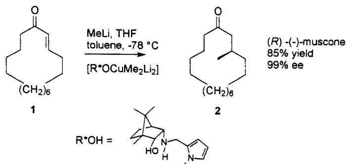
Scheme 7.3. Asymmetric synthesis of ( R )-muscone.
