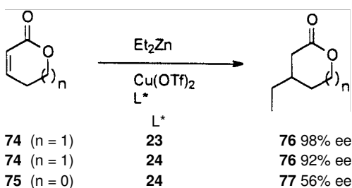
Scheme 7.21. Enantioselective conjugate addition to lactones.
