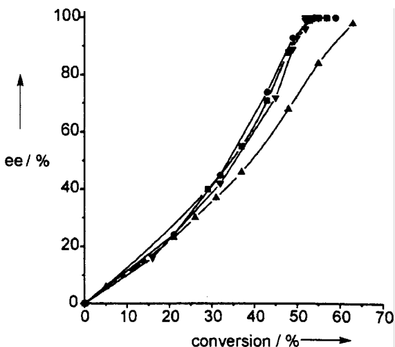
Fig. 7.9. Ee against conversion for the kinetic resolution of 53 with ( S , R , R )- 18 , Cu(OTf) 3 , and Et 2 Zn (■), i Pr 2 Zn (▲), n Bu 2 Zn (●), and Me 2 Zn (▼).
