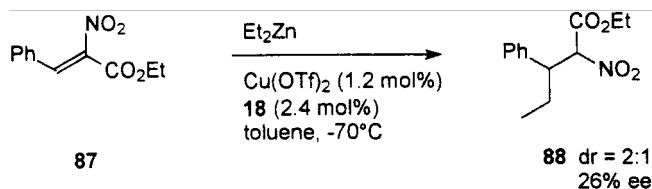
Scheme 7.23. Enantioselective conjugate addition to \alpha, \beta -unsaturated nitroacetates 87 .
