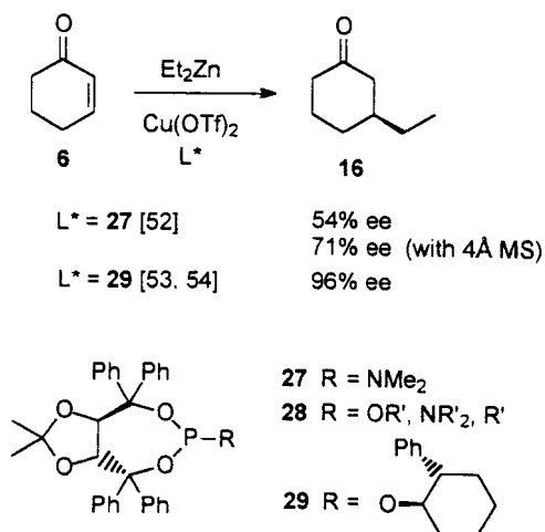
Scheme 7.13. TADDOL-based phosphoramidite ligands in the catalytic 1,4-addition.
