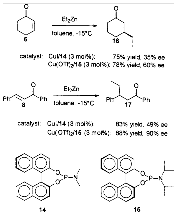
Scheme 7.9. Copper-catalyzed 1,4-addition to cyclohexenone and chalcone, with phosphoramidites as chiral ligands.
