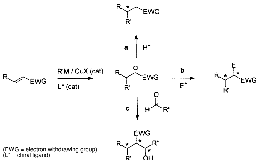
Scheme 7.1. Catalytic conjugate addition and tandem conjugate addition.
