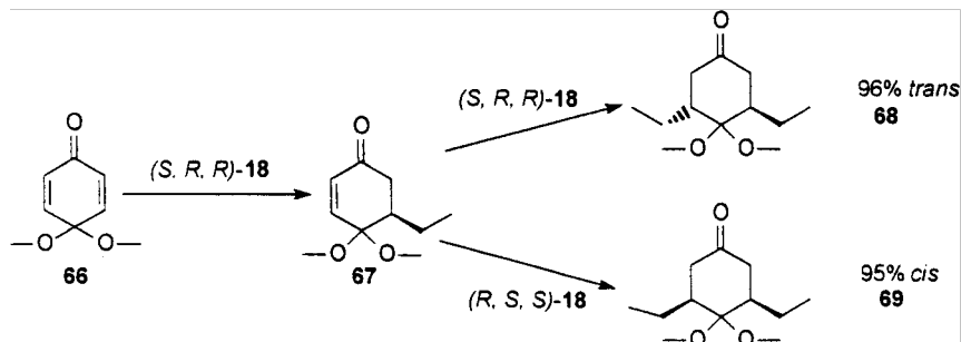
Scheme 7.18. Selective cis or trans double conjugate addition of Et 2 Zn to cyclohexadienone monoacetal 66 .
