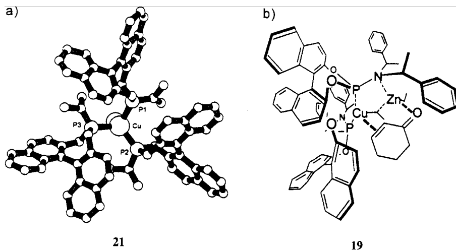
Fig. 7.3. a) X-ray structure of the CuI complex 21 of ligand 14 ; b) Possible bimetallic intermediate involved 19 in si -face-selective ethyl transfer to 2-cyclohexenone.
