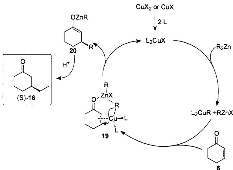
Scheme 7.12. Catalytic cycle for 1,4-additions of \text{R}_2\text{Zn} reagents.
