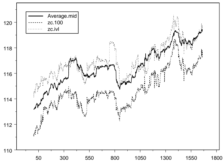
Figure 8: Theoretical values and average quote Ahold 3% (top) and Ahold 4% (bottom) (zero-coupon interest structure).
