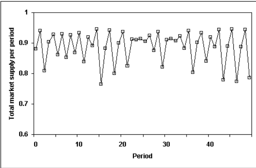
Fig. 6.9 Chaotic market supply, c=0.05 , a=18 , initial value 0.81.
