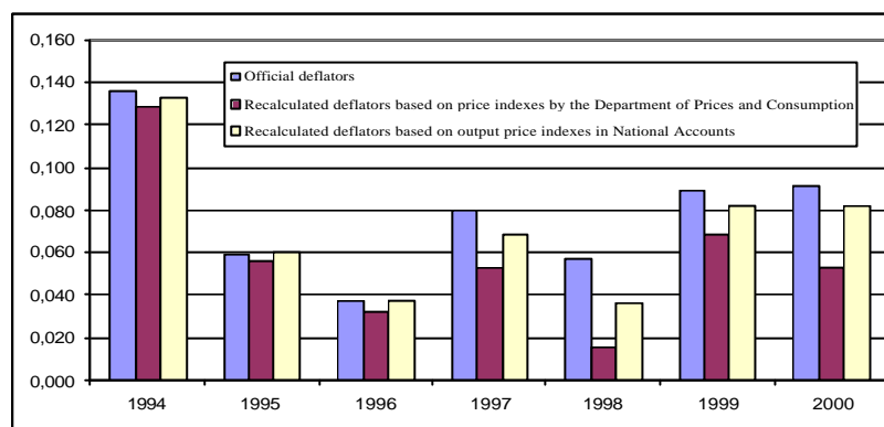
Figure 15 Labor productivity growth rates in the total manufacturing industry with official and recalculated deflators
