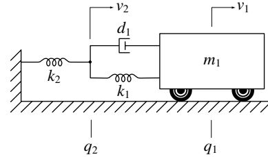
Fig. 3. Example system for mechanical co-content.
