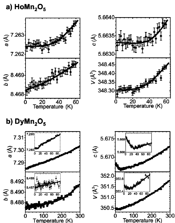
FIG. 2. Lattice parameters and unit cell volumes of \text{HoMn}_2\text{O}_5 and \text{DyMn}_2\text{O}_5 as a function of temperature.
