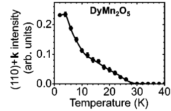
FIG. 4. Integrated intensity of (100) +\mathbf{k} magnetic Bragg peak as a function of temperature for DyMn 2 O 5 .
