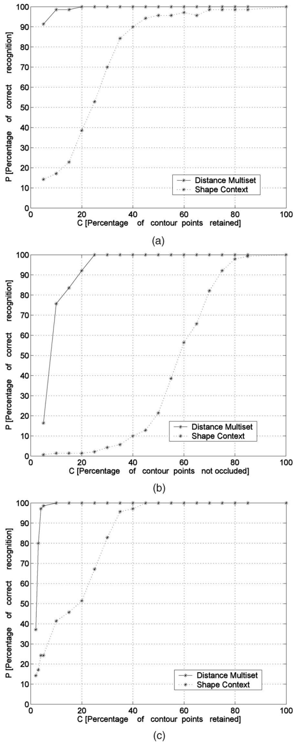
Fig. 6. Results of the ICR tests with a subset of MPEG-7 data set: (a) Segment-wise deletion test: The distance multiset method gives 100 percent recognition rate when more than 20 percent of the contour is retained. The shape context method performs reasonably well (more than 90 percent recognition rate) when more than 40 percent of the contour points are retained. (b) Occlusion test: The shape context method is particularly affected by occlusion because the shape context descriptors of contour points near the occlusion boundary are radically different from the shape contexts of the points in the complete contours. (c) Depletion test: The distance multiset method and the shape context method perform very well for more than 5 percent and 40 percent retention of contour pixels.
