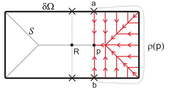
Fig. 2. A rectangle shape \Omega , its skeleton \mathcal{S} , the root R , a skeleton point p , and p 's feature points a, b . The collapse of p is formed by the origins of the trajectories (red) through p .
