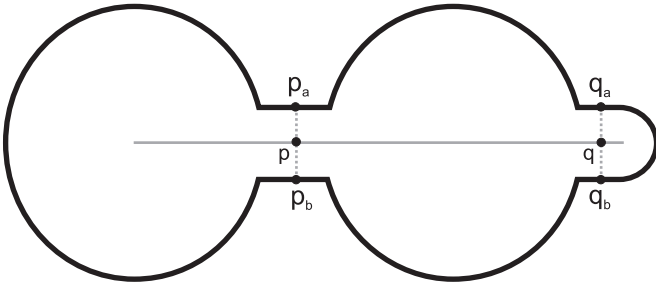
Fig. 1. A 2D shape and its skeleton. Points p, q \in \mathcal{S} and their feature points p_a, p_b and q_a, q_b respectively have locally identical configurations. Globally however, p is considered more important than q .
