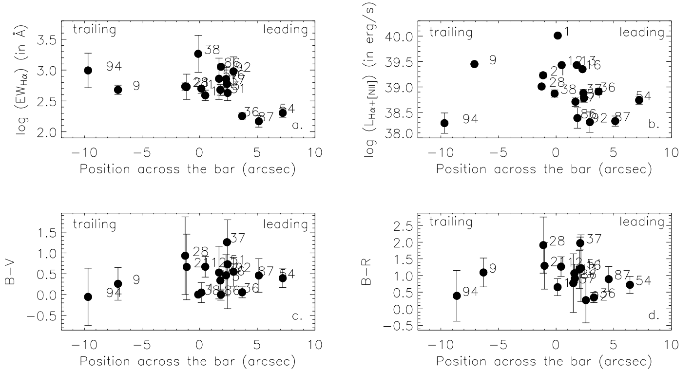
Fig. 7. Representation of (from top to bottom and from left to right) the H\alpha equivalent width ( EW_{H\alpha} ), H\alpha+[N II] luminosity, and B - V and B - R broad-band colours of the bar H II regions of NGC 1530 as a function of their projected distance from the bar dust-lane in arc seconds. Zero means that the H II region is located on the bar dust-lane, negative and positive values refer to H II regions located on the trailing and leading side of the bar dust-lane respectively. The EW_{H\alpha} have been corrected for [N II] contamination as described in Sect. 2.3. The broad-band colours have only been corrected for Galactic extinction (Schlegel et al. 1998).
