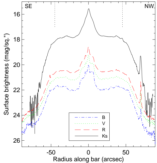
Fig. 3. Surface brightness profile along the major axis of the bar (PA= 121^\circ ) of NGC 1530 for the B, V, R and Ks bands. The data were corrected for Galactic extinction (Schlegel et al. 1998). The dotted line indicates the approximate location of the bar end.
