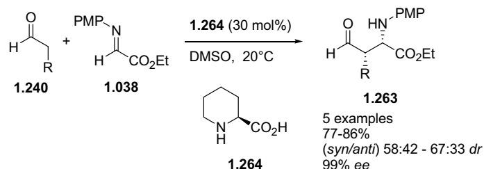
Scheme 1.68. Mannich reaction catalyzed by pipecolic acid.
