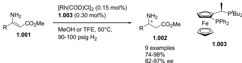
Scheme 1.02. Rhodium-ferrocenylphosphine catalyzed hydrogenation of unprotected enamines.
