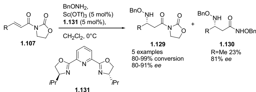
Scheme 1.37. Sc-catalyzed addition of benzylhydroxylamine to oxazolidinones.
