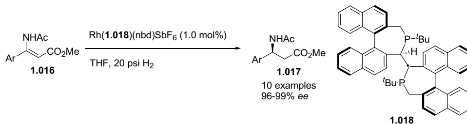
Scheme 1.07. Rhodium-bisphosphepine catalyzed hydrogenation of ( Z )-enamines using bisphosphepine lignds.
