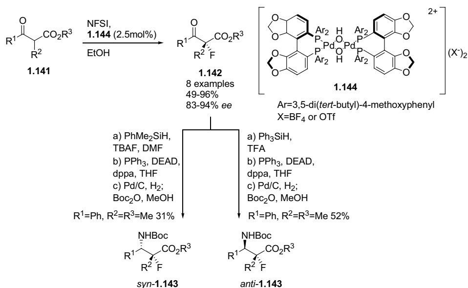
Scheme 1.40. \text{Pd} -catalyzed enantioselective fluorination of \beta -ketoesters.
