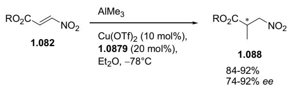
Scheme 1.25. Cu-catalyzed addition of trimethyl aluminium to a nitro-olefin.
