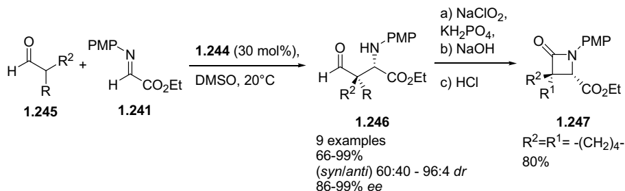
Scheme 1.62. Proline catalyzed asymmetric Mannich reaction to form quaternary all carbon stereocenters.
