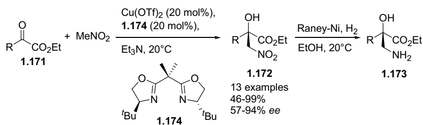
Scheme 1.47. Cu-catalyzed asymmetric Henry reaction.
