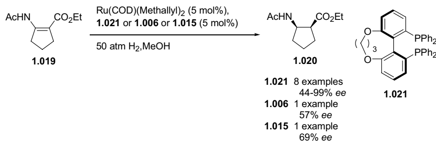
Scheme 1.08. Ru-catalyzed hydrogenation towards cyclic \beta -amino acids.
