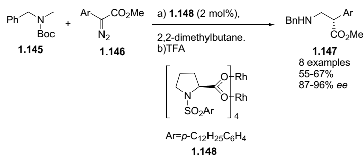
Scheme 1.41. \text{Rh} -catalyzed C-H activation for the synthesis of \beta^2 -amino acids.
