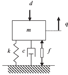
Fig. 1. Mass-spring-damper system.
