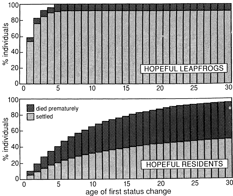
FIG. 7.—Cumulative frequency of settling and of premature death of hopeful residents ( bottom ) and hopeful leapfrogs ( top ) at the evolutionary stable relative frequency of hopeful leapfrogs obtained from eq. (15).
