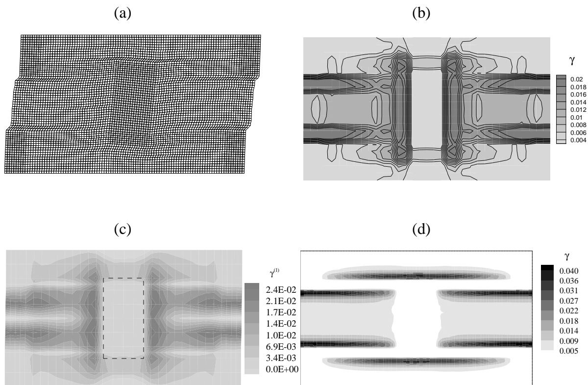
Figure 5: Deformation fields for the composite under simple shear (see inset) according to various theories: (a) deformed mesh (amplified) according to discrete dislocation plasticity (from [11]); (b) slip distribution according to the Acharya-Bassani theory (from [16]); (c) idem according to Gurtin's nonlocal theory [17] and (d) idem according to Groma's theory [15].
