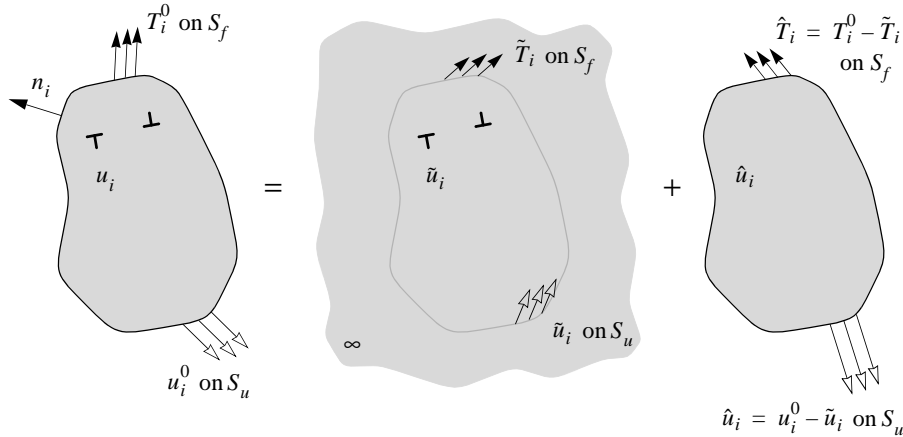
Figure 2: Decomposition into the problem of interacting dislocations in the infinite solid ( \tilde{\cdot} fields) and the complementary problem for the finite body without dislocations ( \hat{\cdot} or image fields).
