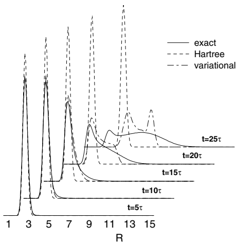
Fig. 6.1. Time-evolution (in units of optical cycles \tau ) of the nuclear density N(R, t) obtained for a one-dimensional model \text{H}_2^+ -molecule in a \lambda = 228 nm, I = 5 \times 10^{13} W/cm 2 laser field from the exact solution, the time-dependent Hartree approximation and a time-dependent correlated variational approach
