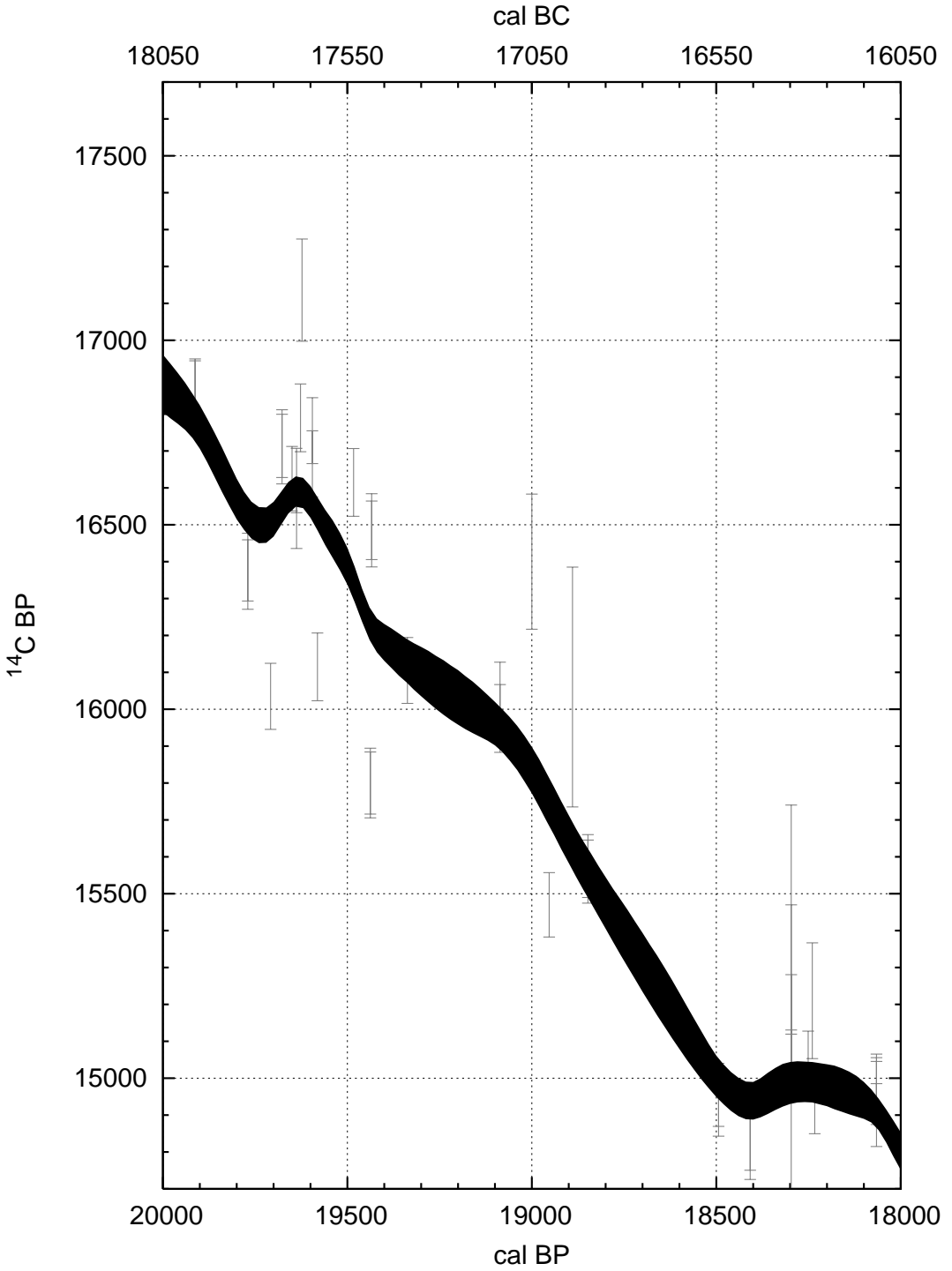
Figure A4 The IntCal04 terrestrial calibration curve (1-standard deviation envelope) and data with 1-standard deviation error bars in 14 C increased by the laboratory error multipliers described in the text. The uncertainty in the calendar ages is not shown, but is taken into account in the random walk model.
