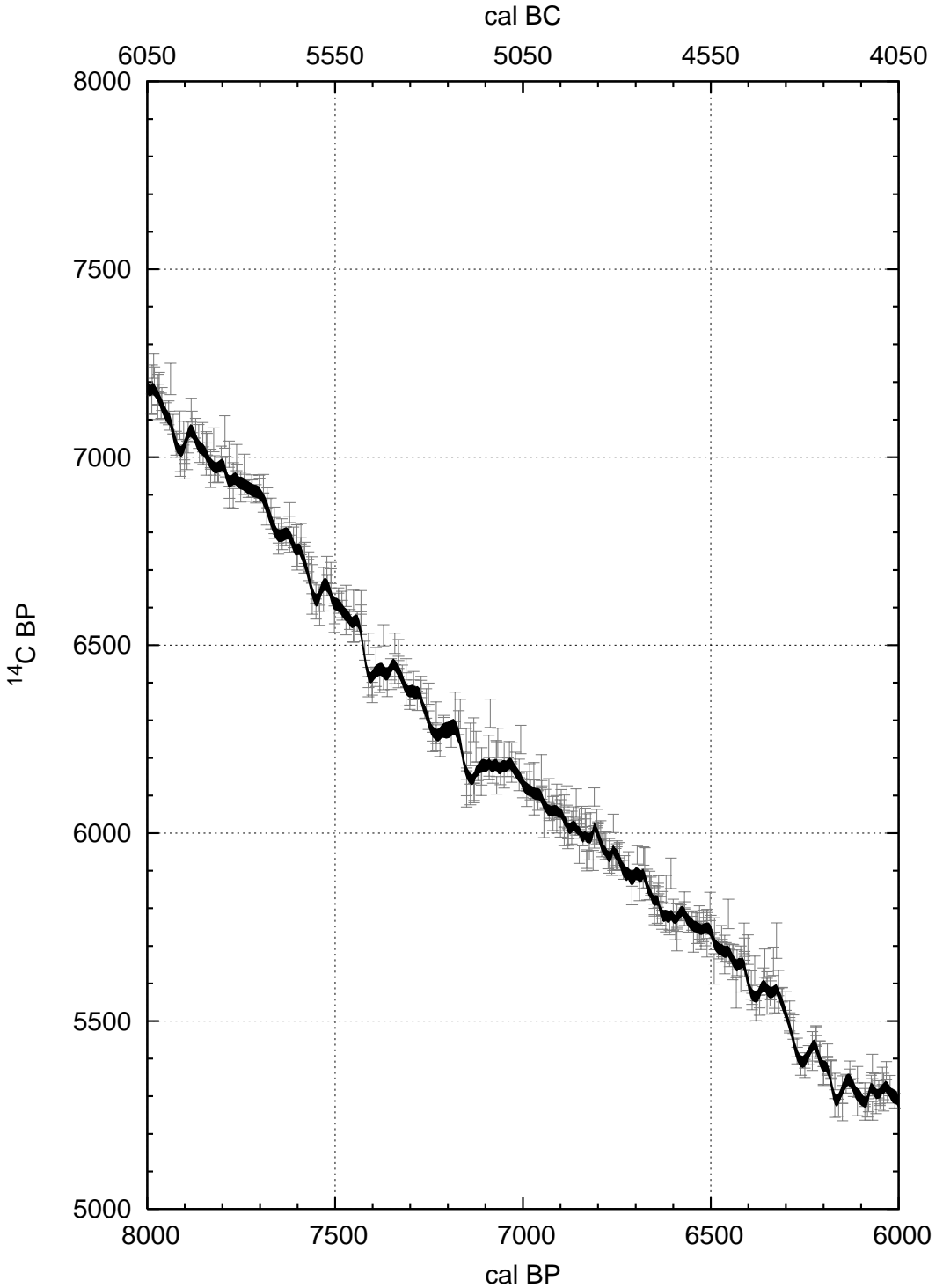
Figure A10 The IntCal04 terrestrial calibration curve (1-standard deviation envelope) and data with 1-standard deviation error bars in 14 C increased by the laboratory error multipliers described in the text. The uncertainty in the calendar ages is not shown, but is taken into account in the random walk model.
