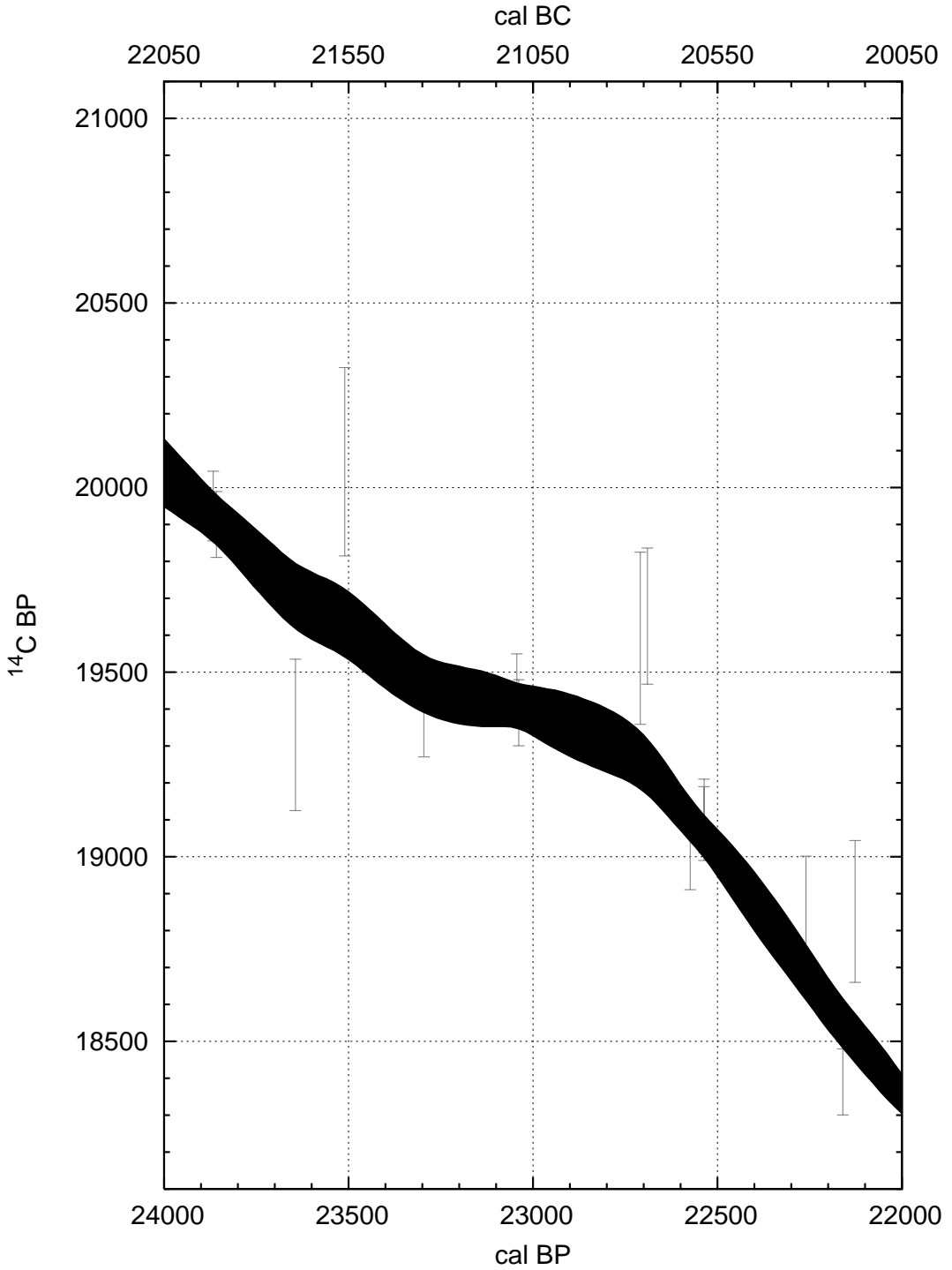
Figure A2 The IntCal04 terrestrial calibration curve (1-standard deviation envelope) and data with 1-standard deviation error bars in 14 C increased by the laboratory error multipliers described in the text. The uncertainty in the calendar ages is not shown, but is taken into account in the random walk model.
