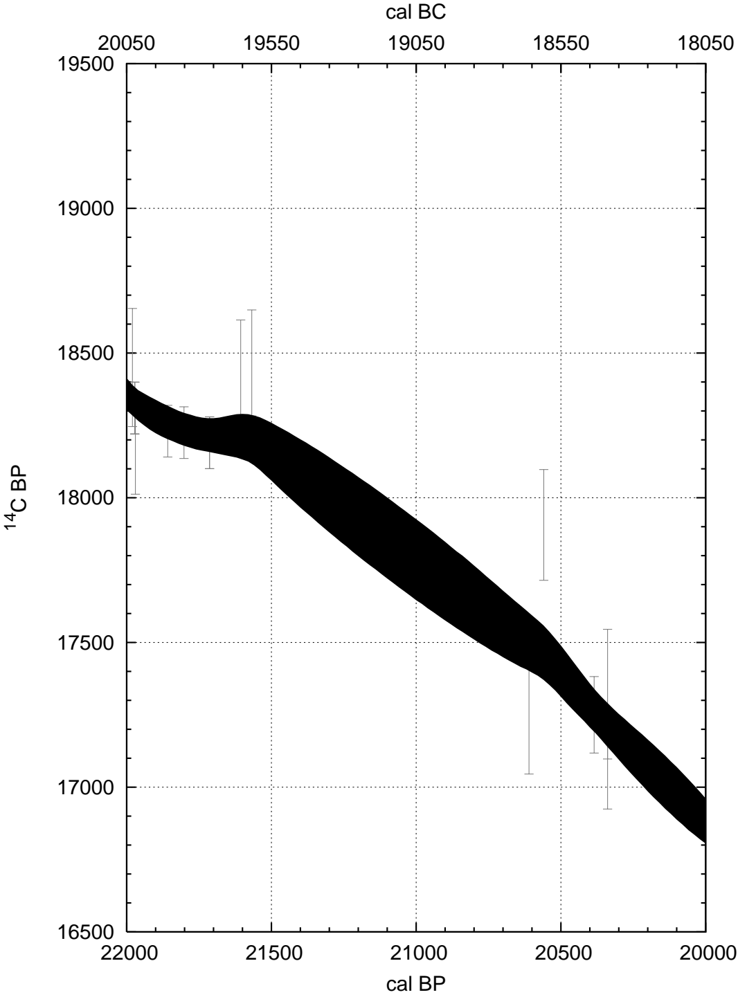
Figure A3 The IntCal04 terrestrial calibration curve (1-standard deviation envelope) and data with 1-standard deviation error bars in 14 C increased by the laboratory error multipliers described in the text. The uncertainty in the calendar ages is not shown, but is taken into account in the random walk model.
