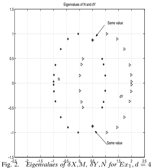
Fig. 2. Eigenvalues of \delta X, M, \delta Y, N for E_{x_1}, d = 4
