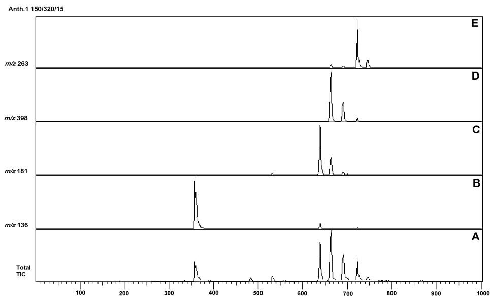
Fig. 2. Representative total GC-MS chromatogram of an A. sylvestris (L.) Hoffm. specimen, collected from location 8 (A). The other chromatograms are extracted ion currents; for the I.S. (B), yatein (C), Deoxy-podophyllotoxin (D) and anhydro-podorhizol (E). On the x-axes the scan-number and on the y-axes the % intensity of selected ion are given.
