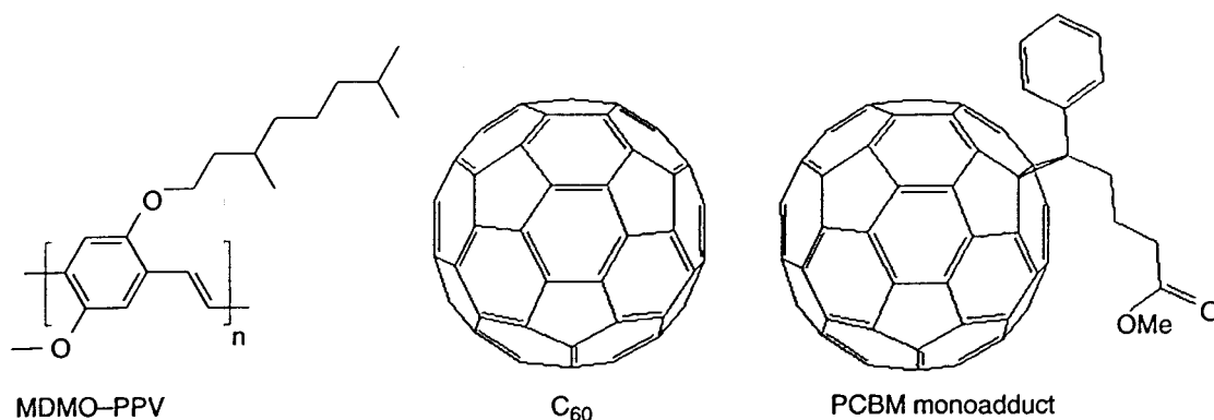
Fig. 1. Molecular structures of MDMO-PPV, C_{60} and PCBM monoadduct. PCBM multiadduct has the same functionalised side groups as PCBM monoadduct, but contrary to PCBM monoadduct it has between two and three side groups.
