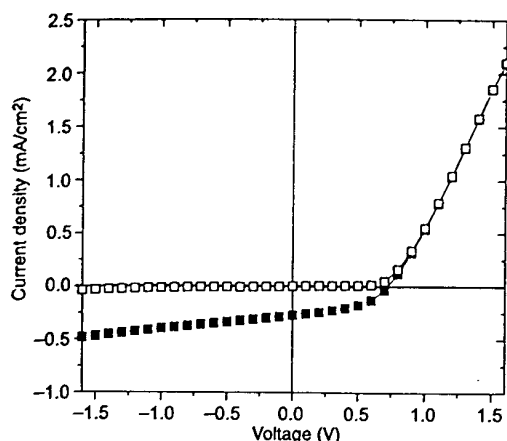
Fig. 4. I-V-behaviour of a 10 \times 15 \text{ cm}^2 MDMO-PPV/PCBM monoadduct) solar cell with an active area of 50 \text{ cm}^2 under light (solid squares) and in the dark (open squares). Illumination is provided by white light from a fluorescence tube with an intensity of 6 \text{ mW/cm}^2 .
