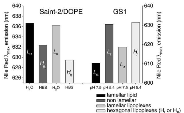
Fig. 3. Phase transition of SAINT-2/DOPE and GS1 lipoplexes as monitored by Nile Red. The \lambda_{\max} emission of Nile Red in GS1 lipoplexes at pH 7.5 and 5.4 was compared to that in SAINT-2/DOPE lipoplexes in water ( H_2O ) and in salt (HBS). Note that a transition from lamellar L_{\alpha} to inverted hexagonal H_{II} phase, as occurs for SAINT-2/DOPE lipoplexes, translates into a decrease in \lambda_{\max} emission. In contrast, a transition from a lamellar L_{\alpha} to a normal hexagonal H_I phase translates into an increase in \lambda_{\max} emission.
