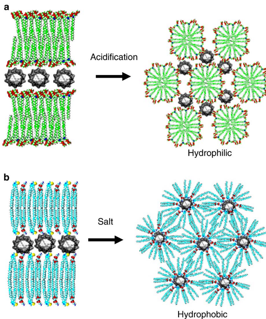
Fig. 6. Model for the phase transition of lipoplexes formed from sugar-based gemini surfactants (a); comparison with SAINT-2/DOPE (b). The model depicted here for the gemini lipoplexes (a) illustrates a transition from a lamellar phase L_{\alpha} to a normal hexagonal H_I phase as presumably occurs in the endosomal compartment upon acidification. In such a H_I phase, the plasmid DNA is intercalated between micelles where the polar head group of the amphiphile is exposed on the outside, giving rise to externally hydrophilic particles. In (b) the lamellar L_{\alpha} organization of SAINT-2/DOPE in the absence of salt and the inverted hexagonal H_{II} phase in its presence is displayed. In this H_{II} phase the polar head groups of the amphiphiles interact with the plasmid DNA and the hydrophobic tails are exposed on the outside, giving rise to externally hydrophobic particles that will tend to aggregate.
