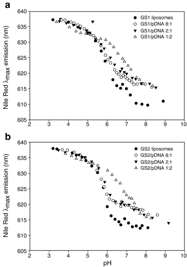
Fig. 2. Lamellar-to-micellar phase transition of sugar-based gemini liposomes and lipoplexes upon acidification. The maximum emission wavelengths ( \lambda_{\max} emission) of Nile Red in GS1 (a) and GS2 (b) liposomes and lipoplexes were determined as a function of pH. In complexes with plasmid DNA, molar charge ratios ( \pm ) of 8:1 2:1 and 1:2 were tested (GS1/pDNA and GS2/pDNA 8:1; 2:1 and 1:2, respectively). Note that upon acidification the \lambda_{\max} emission of Nile Red increases consistent with its exposure to a more polar microenvironment and the conversion of the gemini lipoplexes to a normal micellar phase.
