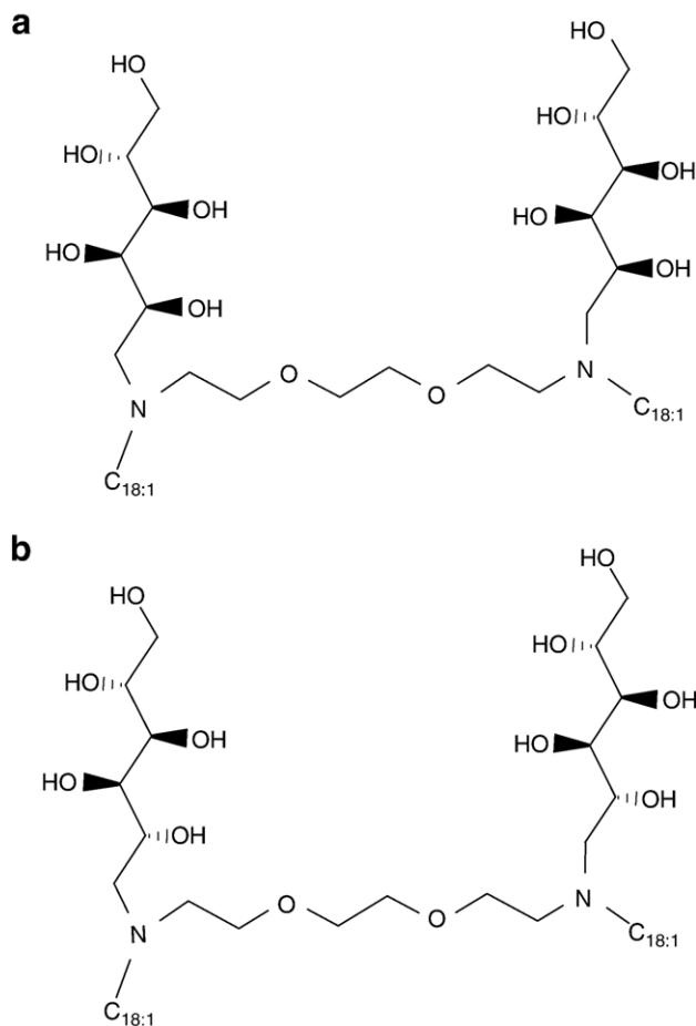
Fig. 1. Chemical structures of GS1 (a) and GS2 (b). The basic structures of the sugar-based gemini surfactants GS1 and GS2 consist of two single-tail surfactants with a reduced sugar and a pH sensitive amino moiety in the headgroup and an oleyl chain as hydrocarbon tail. Both twin structures are linked via an ethylene oxide spacer between the two tertiary nitrogens. GS1 (a) and GS2 (b) differ by the nature of the reduced sugar, glucose and mannose, respectively. Note that the degree of protonation of the two nitrogens within the sugar-based gemini surfactant is dependent on pH. Consequently, these amphiphiles are fully charged at mildly acidic pH.
