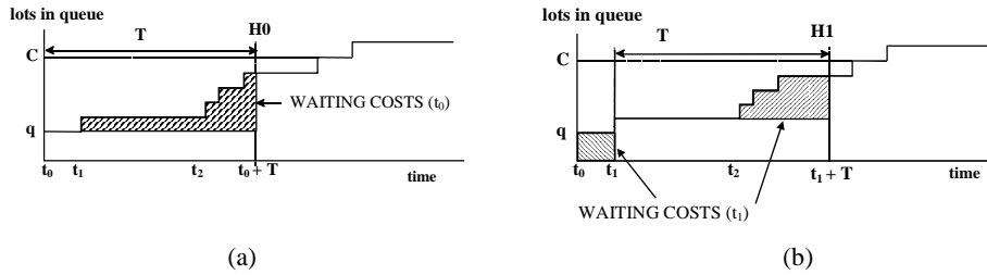
Figure 3a,b: Starting the batch machine at t_0 causes waiting costs for the items that arrive during processing ( T ). On the other hand, if the batch machine were to be loaded at t_1 , next to these costs also the waiting costs for items in queue ( q ) at the decision moment ( t_0 ) should be taken into account.
