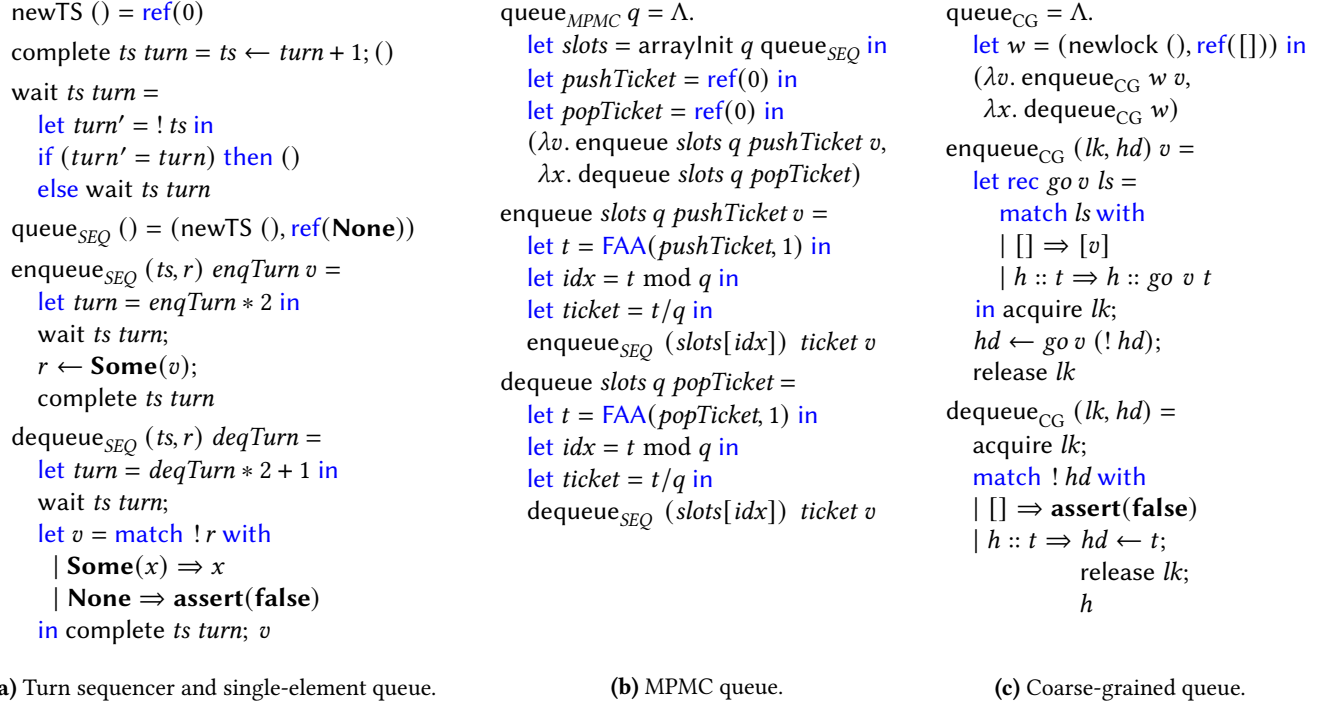
Figure 1. Implementation of the various data structures.
