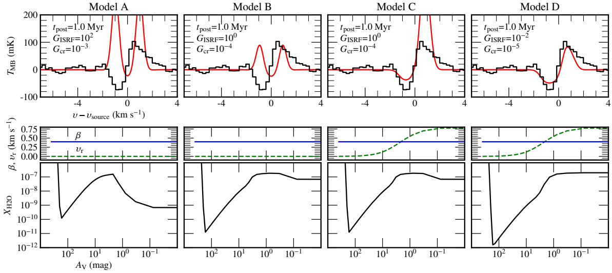
Fig. 20. Illustration how various physical and chemical parameters can be constrained using the SWaN network. \text{H}_2\text{O } 1_{01}-1_{01} 557 GHz observations of the Class I source L1551-IRS5 are compared with SWaN models assuming different parameters for the FUV fluxes and velocity profile. Top row: observations (black) together with the synthetic spectra (red). Bottom row: adopted velocity profile (green) and water abundance profile (with respect to \text{H}_2 ) (black). A constant Doppler broadening of \beta = 0.4 \text{ km s}^{-1} is assumed, whereas the radial velocity profile is either taken to be constant at 0 (Models A and B) or to have an expansion profile (Models C and D). The radiation fields G_{\text{ISRF}} and G_{\text{CR}} strongly decrease from model A to model D. A pre-stellar stage duration of 0.1 Myr is used. Based on Schmalzl et al. (2014).
