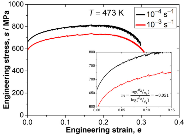
Fig. 2. Tensile stress-strain curves of NbTiZr deformed at 473 K for various strain rates. Enlarged view of the stress-strain curve and strain-rate sensitivity, m was evaluated using the formula shown in the inset.
