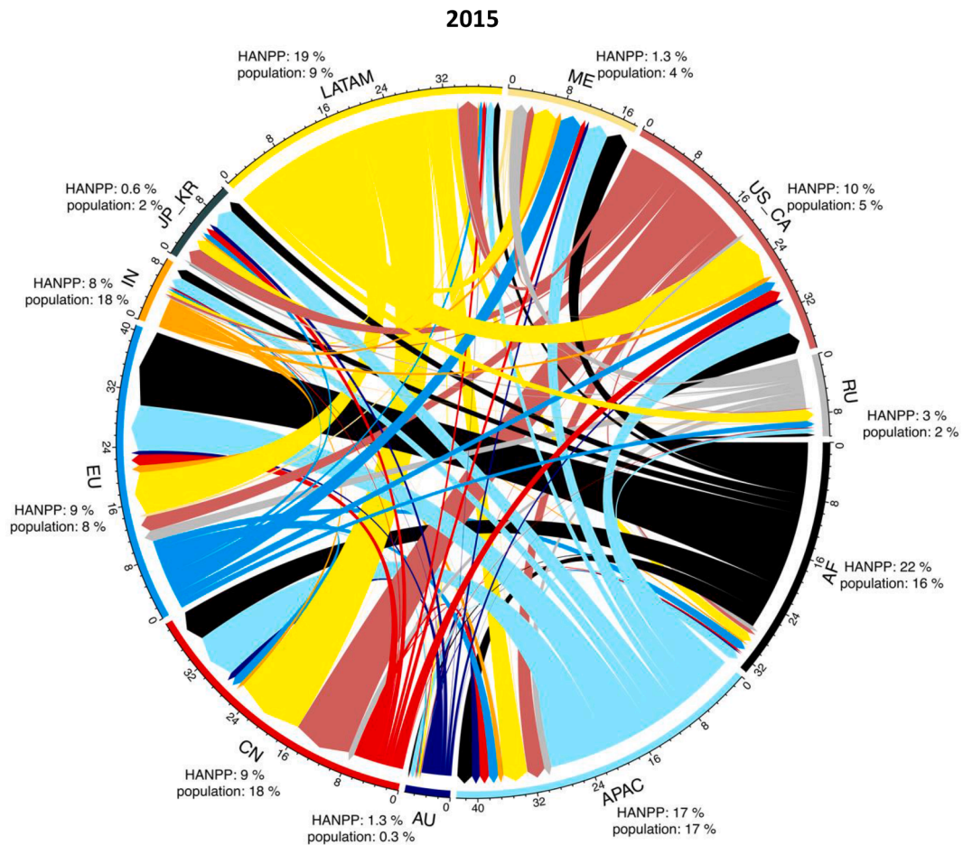
Fig. A2. Embodied HANPP flows between world regions as directed arrows in 2015. Values in the circular network plot are given in exajoules [EJ]. Annotated text gives shares of global HANPP and population respectively. LATAM = Latin America, ME = Middle East, US_CA = USA and Canada; RU = Russia, AF = Africa, APAC = Asia and Pacific, AU = Australia, CN = China, EU = Europe, IN = India, JP_KR = Japan and South Korea.
