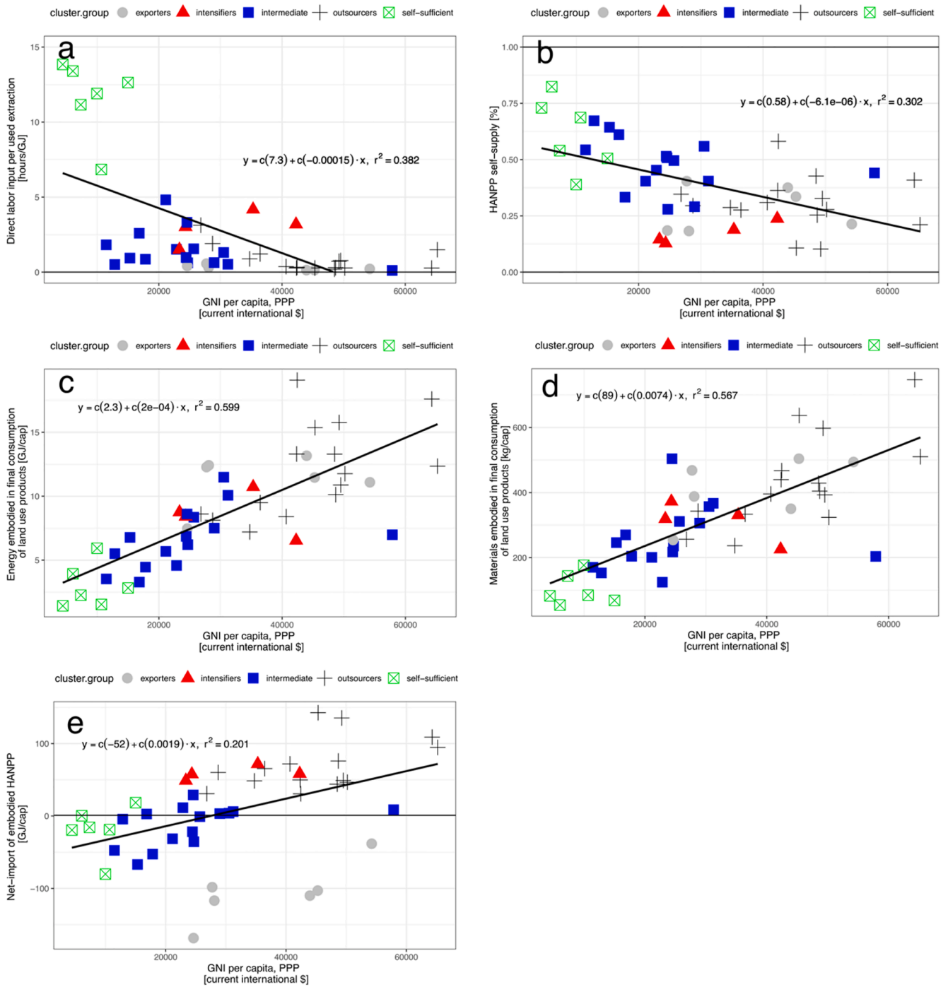
Fig. 4. Linear regression analyses (two-sided test) with GNI per cap (PPP, current international $) as the predictor (year = 2015). With increasing income countries tend to use less direct labor input for appropriating NPP and have a lower HANPP self-supply (a and b). With income increasing, countries tend to have a higher energy and material footprint associated with their biomass consumption (c and d). Richer countries also tend to net-import more eHANPP (e). Predictor (4a-e): mean = 31,348; sd = 15,744. 4a) respondent: mean = 2.56; sd = 3.82; F = 27.19. 4b) respondent: mean = 0.39; sd = 0.17; F = 19.05. 4c) respondent: mean = 8.73; sd = 4.15; F = 65.69. 4d) respondent: mean = 319.72; sd = 154.25; F = 57.56; 4e) respondent: mean = 7.51; sd = 66.70; F = 11.10. All regressions are significant at a p-value < 0.01. N = 46, df: 44.
