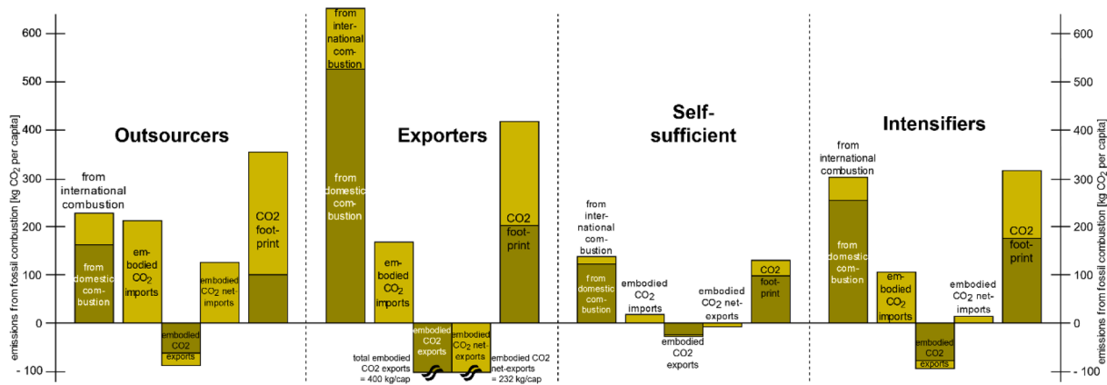
Fig. A6. Barplots indicating embodied CO 2 emission flows from combustion which are due to the economic activities of the land-use system for the year 2015. That is, the CO 2 emissions occurring from combustion to appropriate domestic NPP and those embodied in traded biomass. The first stacked bar of each group distinguishes the origin of the emissions occurring from domestic biomass production (domestic vs. international). The subsequent bars show the emissions embodied in biomass imports and exports. Their subtraction yields the net-trade and finally the footprint, which are the domestic emissions plus net-trade. Note that each bar captures the same process, i.e., the first bar of each group presents the process of NPP appropriation and the emissions involved, the second row the biomass imports and the emissions embodied in those imports, etc. All values are given on per capita levels. The share of domestic emissions exported is calculated by assuming an equal distribution of domestic and international emissions for domestic consumption and exports.
