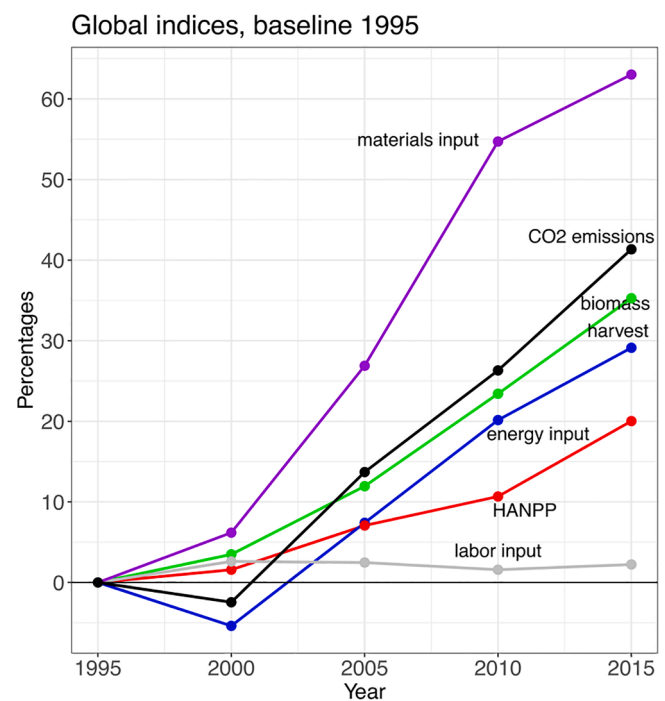
Fig. 1. Index development of biomass harvest, HANPP, emissions of CO 2 from combustion, and the inputs of energy, materials, and labor, from 1995 to 2015; base year 1995. Growing energy and materials inputs enabled a relative decoupling from biomass harvest and HANPP and caused an increase in CO 2 emissions from combustion, while labor inputs stagnated on a global level. Note that there is a data point only every 5 years. Years in between are interpolated.
