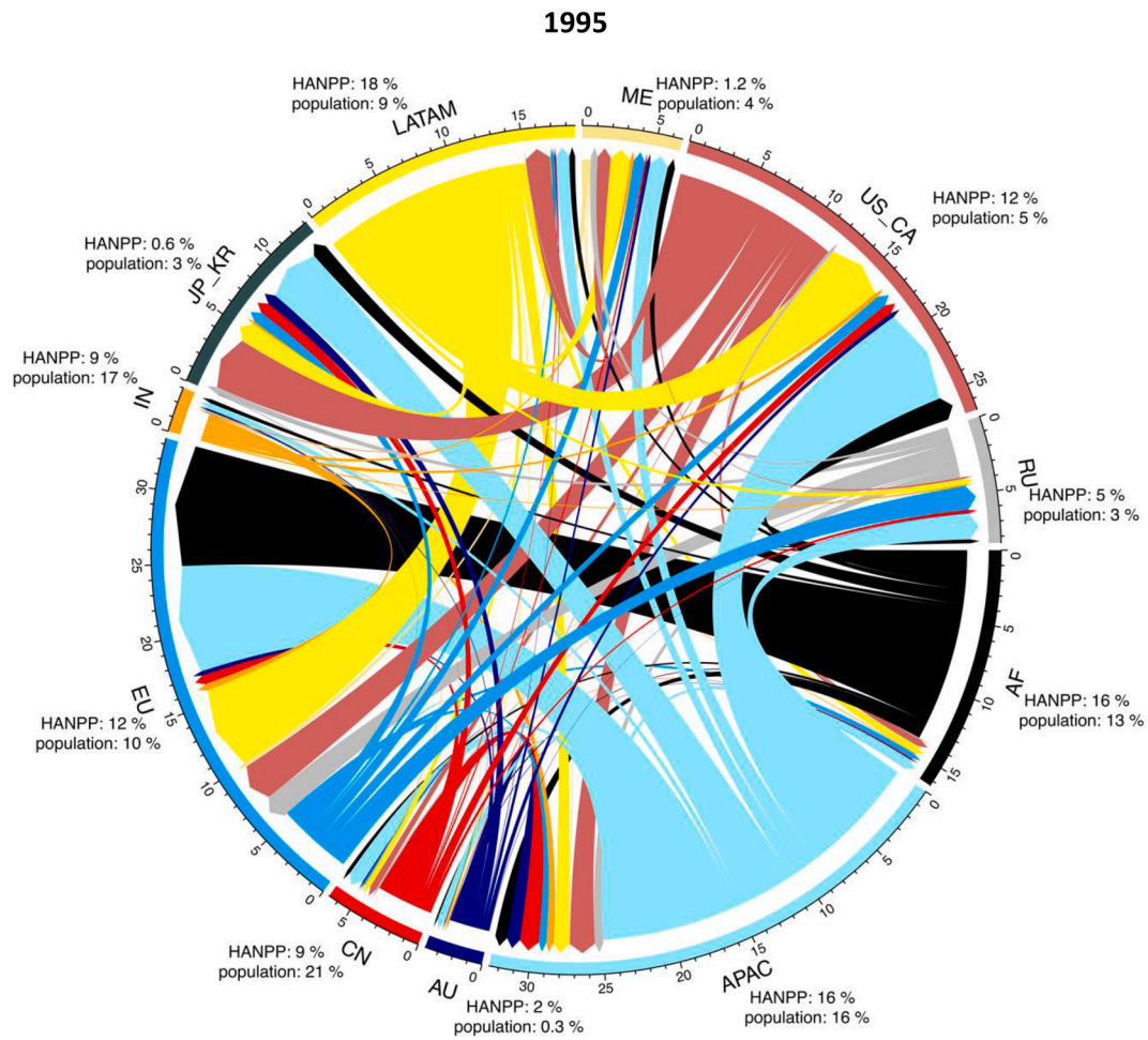
Fig. A1. Embodied HANPP flows between world regions as directed arrows in 1995. Values in the circular network plot are given in exajoules [EJ]. Annotated text gives shares of global HANPP and population respectively. LATAM = Latin America, ME = Middle East, US_CA = USA and Canada; RU = Russia, AF = Africa, APAC = Asia and Pacific, AU = Australia, CN = China, EU = Europe, IN = India, JP_KR = Japan and South Korea.
