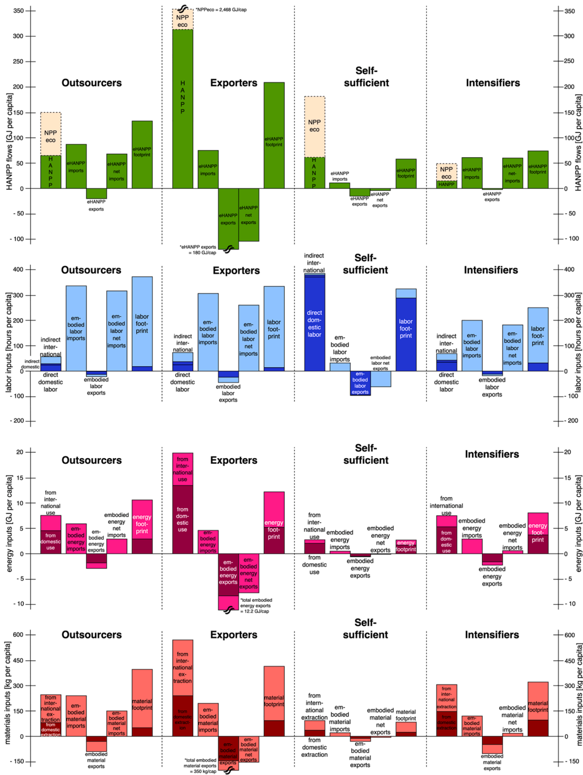
Fig. 5. Barplots indicating HANPP flows and inputs of labor, energy, and materials in the land-use system for the year 2015. Values for the CO 2 emissions and for the intermediate cluster are provided in the appendix. The first row describes the HANPP flows, including domestic HANPP and NPP eco (their sum is NPP pot ), eHANPP trade flows, and the eHANPP footprint. The subsequent rows show the inputs of labor, energy, and materials required to appropriate domestic NPP and those embodied in traded biomass. Materials comprise all fossil materials, metals, and non-metallic minerals used directly or indirectly by the land-use sectors to produce their outputs. The first stacked bar of each group distinguishes the origin of the inputs used for domestic biomass production (domestic vs. international). The subsequent bars show the resources and labor embodied in biomass imports and exports. Their subtraction yields the net-trade and finally the footprint, which is the domestic appropriation plus net-trade. Note that each bar captures the same process, i.e., the first bar of each group presents the process of NPP appropriation and the resources required, the second row the eHANPP imports and the resources embodied in those imports, etc. All values are given on per capita levels. The share of domestic labor, energy, and materials exported is calculated by assuming an equal distribution of domestic and international resources for domestic consumption and exports.
