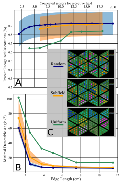
Fig. 5. Receptive fields' topologies: A) Fraction of recognised orientations for each receptive fields' structure, as a function of connected sensing elements (mean and std shaded). B) Minimum detectable angle as a function of bar length (mean and std shaded). C) One example for each of the three topologies.
