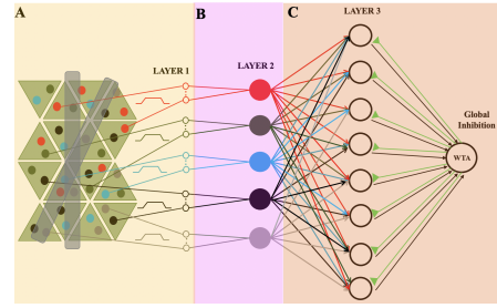
Fig. 1. Spiking neural network for edge orientation: (A) Skin patch from the iCub robot and layer one, which encodes the analog signal into spikes. (B) First order tactile neurons (layer two) gathering the 160 inputs from layer one, organised in receptive fields. (C) Layer three discriminates edge orientation and includes a global inhibitory neuron that implements the WTA network.
