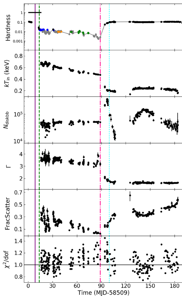
Figure A1. Evolution of the main spectral parameters from the spectral fits with the continuum model \text{TBNEW}*(\text{SIMPL}*\text{DISKBB}) . In the top panel we show the hardness ratio for comparison. From the second panel to the bottom: disc temperature at the inner radius ( kT_{\text{in}} ) in keV, DISKBB normalization ( N_{\text{diskbb}} ), photon index ( \Gamma ), scattered fraction (FracScatter), and the reduced \chi^2 . Same as Fig. 5, we did not plot the data after day 187 (MJD 58596), since that the disc component was not needed in the spectral fits and the spectra can be fitted well with a single power-law with \Gamma \sim 1.6 .
