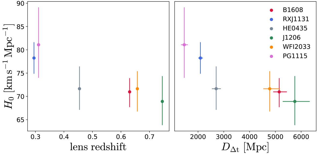
Figure A1. H_0 constraints for the individual H0LiCOW lenses as a function of lens redshift (left) and time-delay distance (right). The trend of smaller H_0 value with increasing lens redshift and with increasing D_{\Delta t} has significance levels of 1.9\sigma and 1.8\sigma , respectively.
