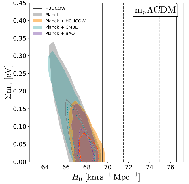
Figure 9. H_0 – \Sigma m_\nu constraint for a m_\nu\Lambda\text{CDM} cosmology. The black contours show the constraints from H0LiCOW alone, while the grey contours show the constraints from Planck alone. The coloured contours show constraints from Planck combined with other probes, as shown in the figure legend. The contour levels represent the 1\sigma and 2\sigma constraints.
