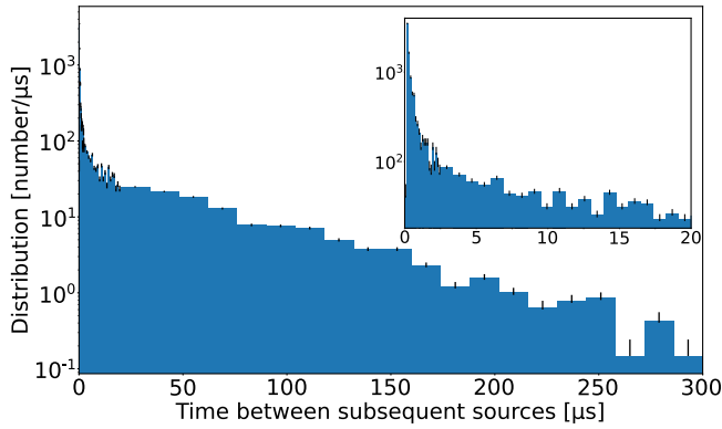
FIG. 2. The distribution of time between subsequent sources. The error bars show the lowest and largest Poisson rates that can model the data with 34% confidence ( 1\sigma ).
