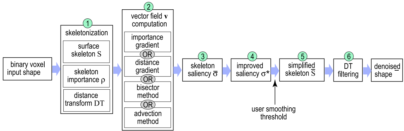
Fig. 10. Pipeline of the proposed feature-preserving smoothing method. See Section 4.
