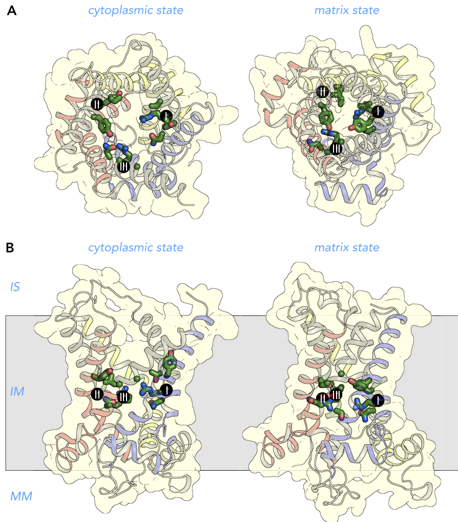
FIGURE 12. Amino acid residues of the substrate binding site View from the intermembrane space (A) and lateral view (B) from the membrane of the human ADP/ATP carrier in the cytoplasmic state (left) and matrix state (right). The structures are described in the legend to FIGURE 7. The black spheres with roman numerals are the contact points of the substrate binding site, which are involved in binding of the substrates (94, 136). Other residues in this site (green) may either bind substrate directly or may allow the binding. IS, intermembrane space; IM, inner membrane; MM, mitochondrial matrix.
