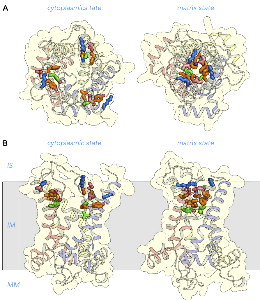
FIGURE 14. Amino acid residues of the cytoplasmic gate
