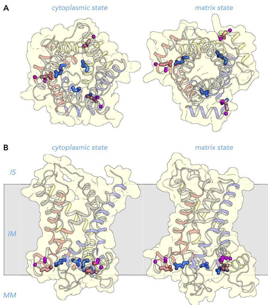
FIGURE 11. Amino acid residues important for the domain structures on the matrix side
