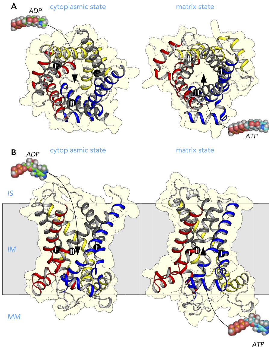
FIGURE 5. Structural changes in the transport cycle of the human mitochondrial ADP/ATP carrier
