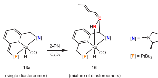
Scheme 11. Reaction of (\text{PNN}')\text{Ru}(\text{H})(\text{CO}) ( 13a ) with 2-Pentenenitrile
