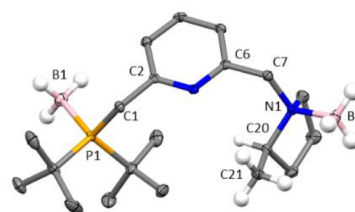
Figure 1. Molecular structure of the bis-borane adduct 7 ( R^1 = R^2 = Me ), showing 50% probability ellipsoids. All hydrogens have been omitted for clarity except for those of the borane groups, as well as those of the CH_3 and CH fragment of the pyrrolidine group. Selected bond lengths: N1–B2 = 1.641(2), P1–B1 = 1.928(2), C6–C7 = 1.514(2), C1–C2 = 1.510(2).
