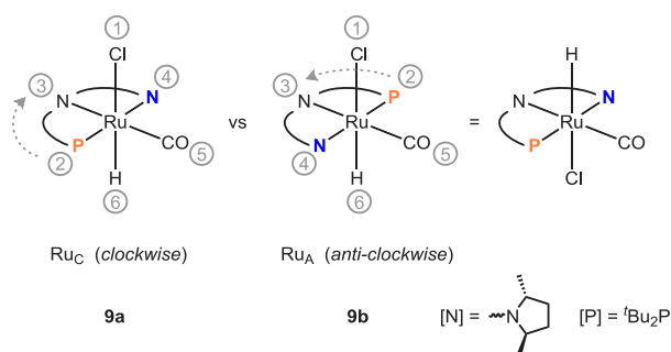
Figure 2. Descriptors clockwise ( Ru_C ) and anticlockwise ( Ru_A ) used to denote the stereochemical configuration around the Ru center in the octahedral (PNN)Ru(H)(CO)(Cl) complexes (ligand priority numbers indicated). Assignment of the stereochemistry of compounds 9a,b is indicated.
