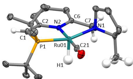
Figure 6. Crystal structure of the dearomatized complex (PNN')Ru(H)(CO) 13a , displayed as 50% ellipsoids.
