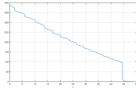
Fig. 8. Time evolution of the PWQ Lyapunov function along the trajectory in Fig. 7.
