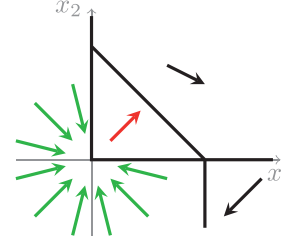
Fig. 4. PWA system whose origin is attractive but where solution starting close to zero can first go away by a certain minimal amount before coming back.
