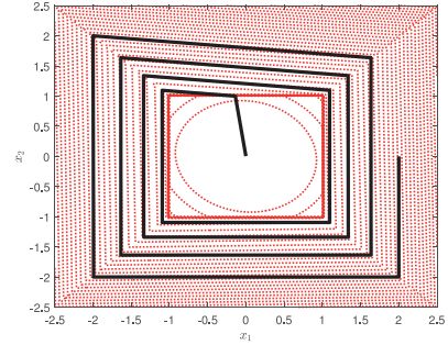
Fig. 7. State space with a trajectory (black line) and the PWQ Lyapunov function level curves (red line).
