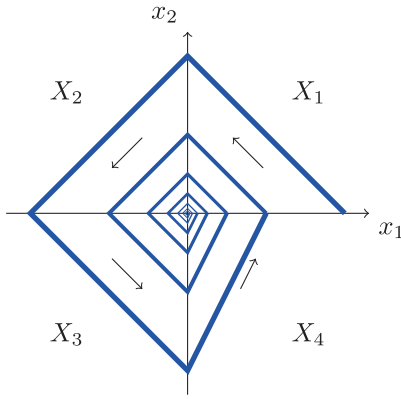
Fig. 2. Planar backward Zeno (Caratheodory) solution (also called left-Zeno solution) reaching the origin. There is no Caratheodory solution starting from the origin. If the flow direction is reversed, the system exhibits a forward Zeno (Caratheodory) solution (also called right-Zeno solution) starting from the origin.
