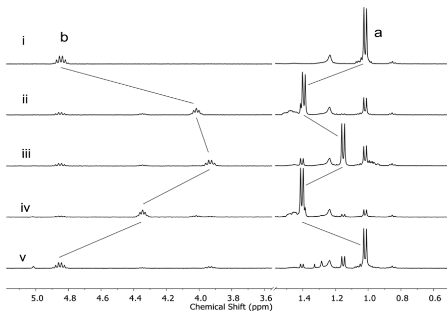
Figure 2. Selected parts of the 1 H NMR spectra of a sample of 1 in DMSO- d 6 ( c = 2.2 \times 10^{-3} M). See Scheme 1 for the atom labeling. (i) E -1 before irradiation. (ii) PSS 365 nm. (iii) 60 °C, 1 h. (iv) PSS 365 nm. (v) 100 °C, 120 min.
