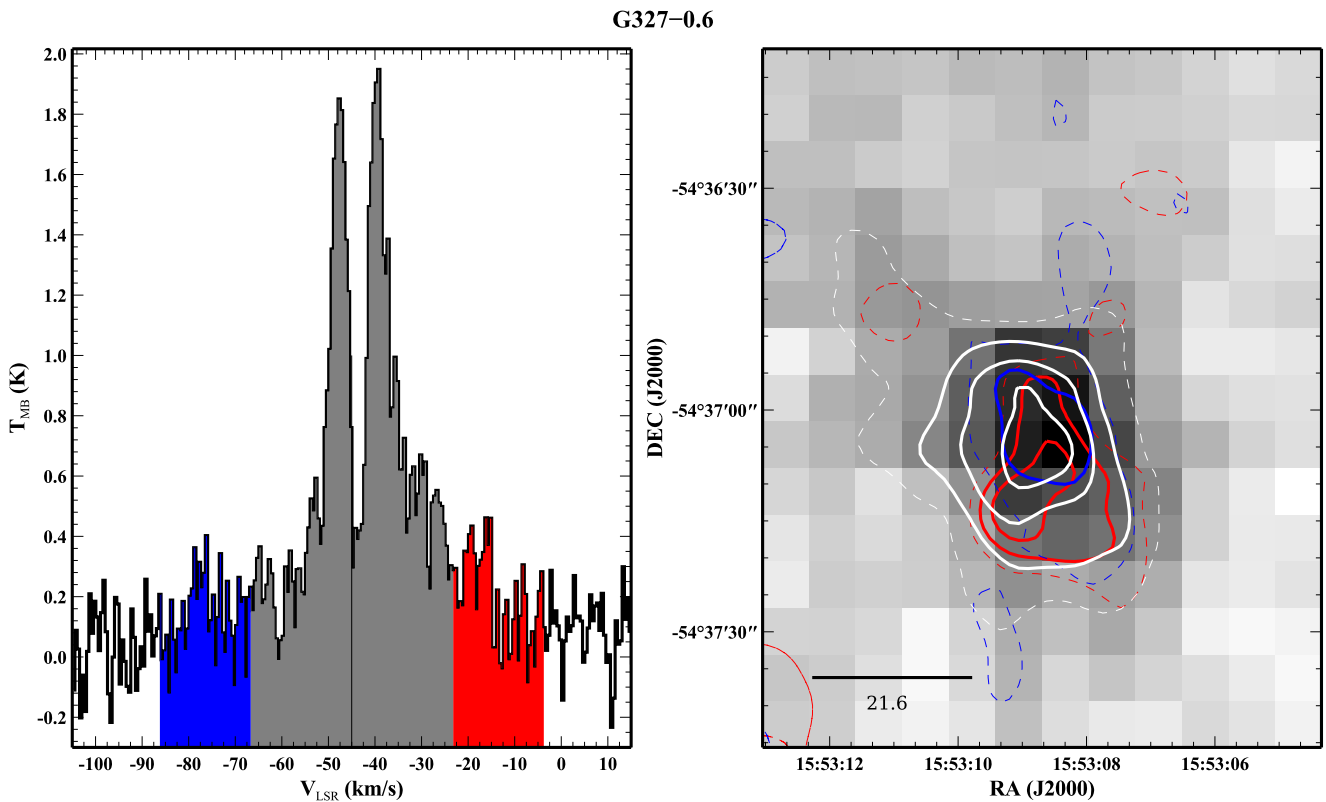
Fig. A.10. As previous figure, for G327.
